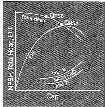
Figure 11: Effect of NPSH on recirculation flow
